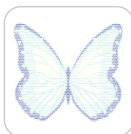
Rasterization
